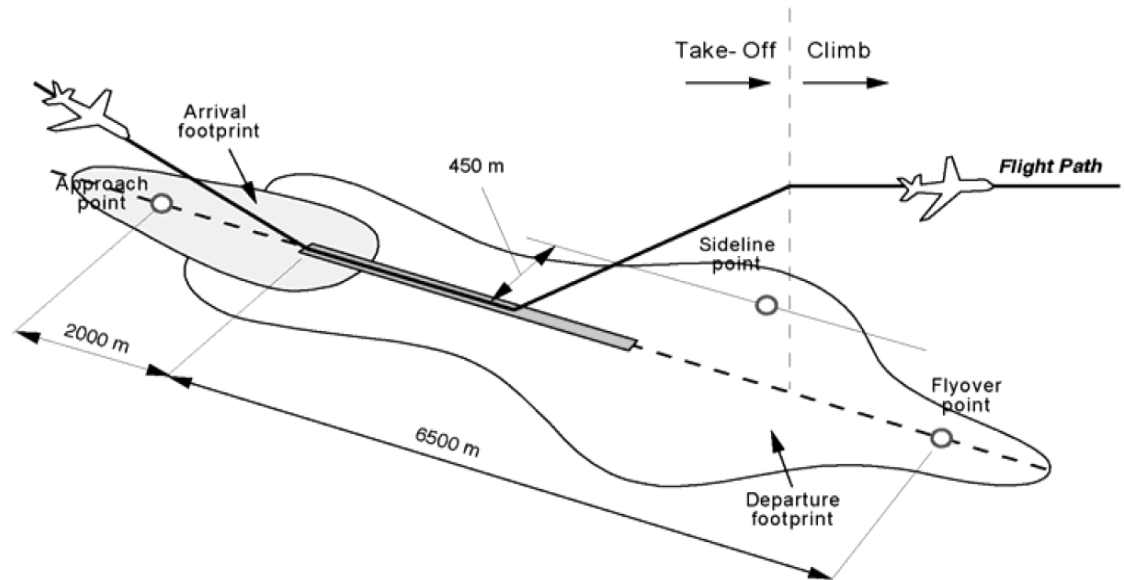
Figure A1.2: Aircraft noise certification measurement points
